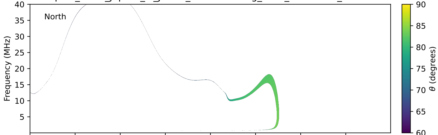
expres_earth_jupiter_io_jrm33_lossc-wid1deg_3kev_20021201_v11.cdf
