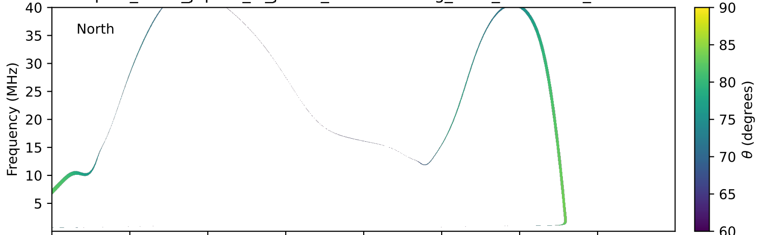
expres_earth_jupiter_io_jrm09_lossc-wid1deg_3kev_20021215_v11.cdf
