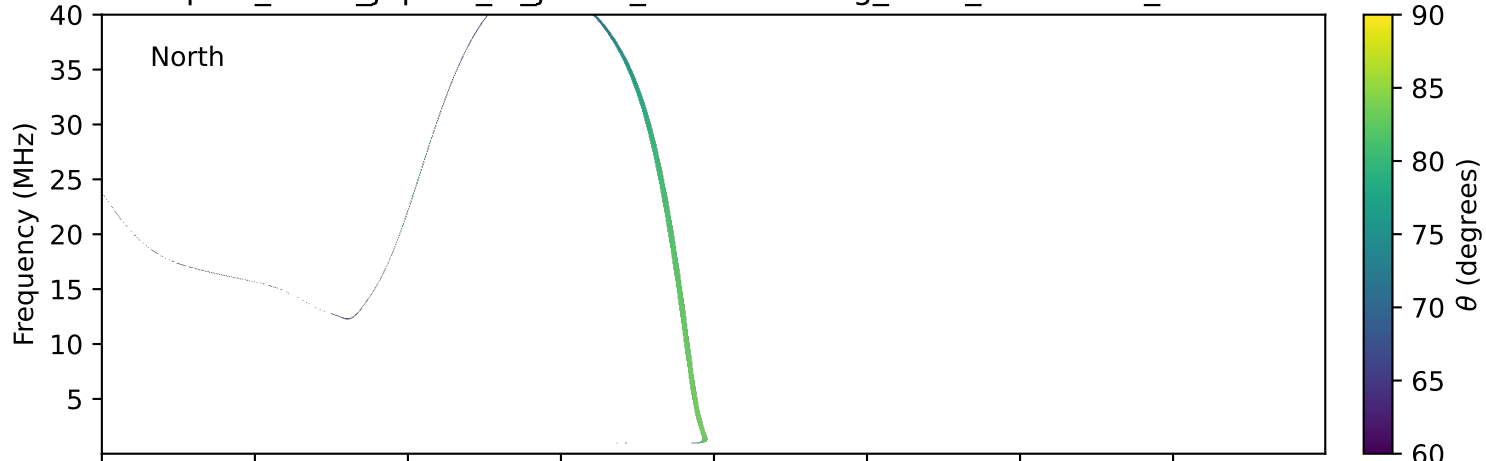
expres_earth_jupiter_io_jrm09_lossc-wid1deg_3kev_20021210_v11.cdf
