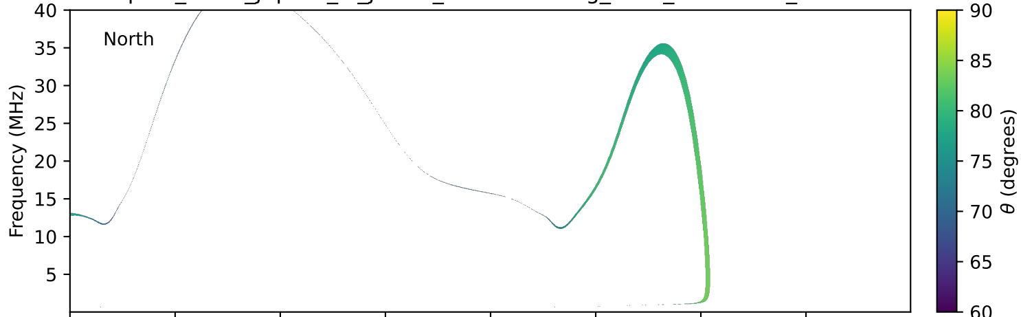
expres_earth_jupiter_io_jrm09_lossc-wid1deg_3kev_20021208_v11.cdf
