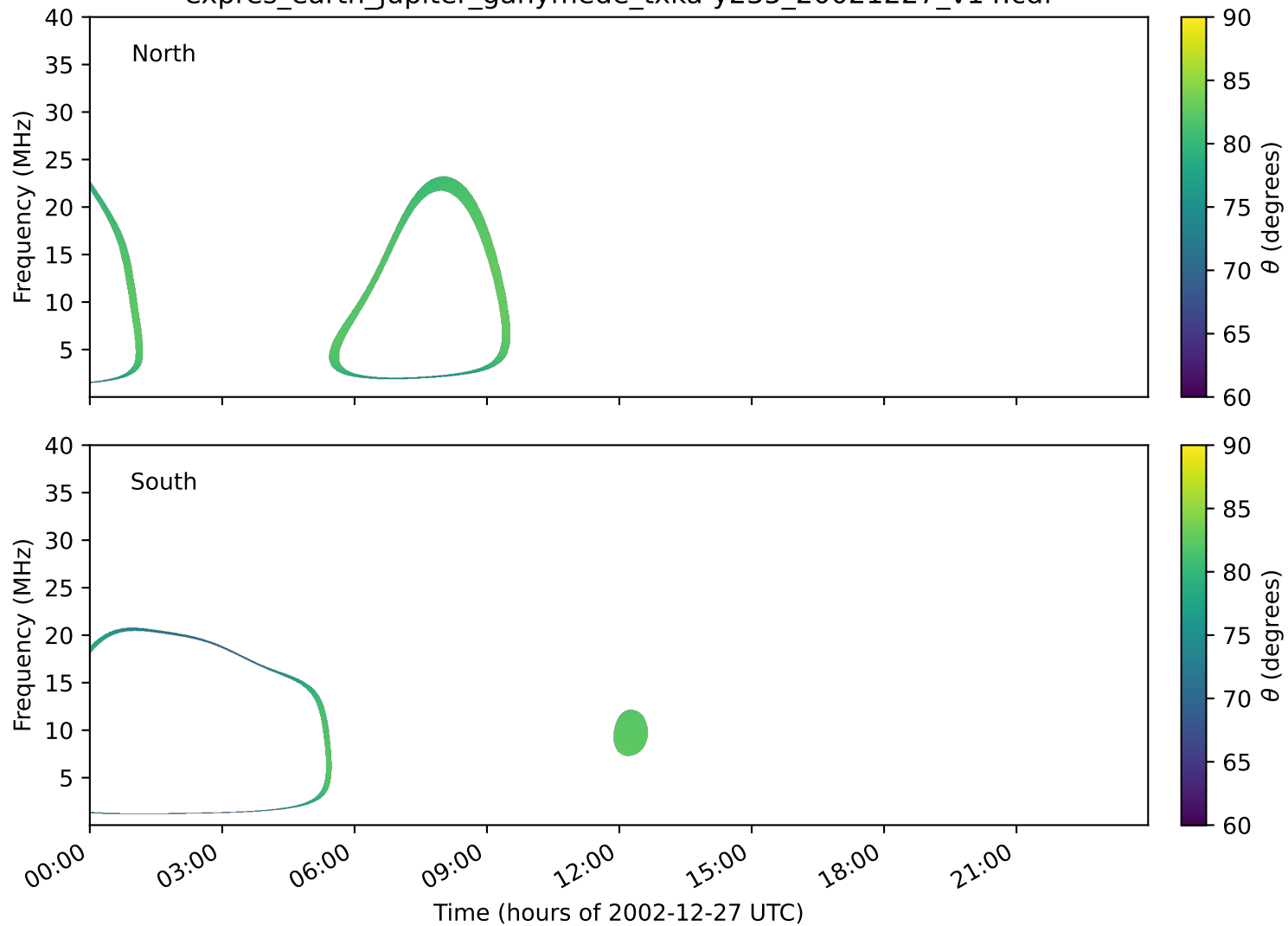
expres_earth_jupiter_ganymede_txka-y235_20021227_v14.cdf
