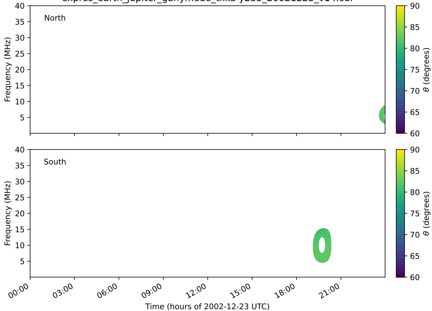
expres_earth_jupiter_ganymede_txka-y235_20021223_v14.cdf
