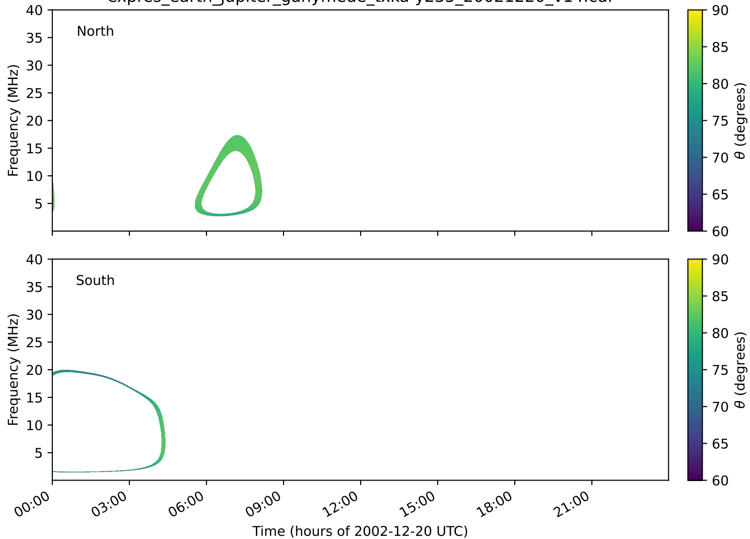
expres_earth_jupiter_ganymede_txka-y235_20021220_v14.cdf
