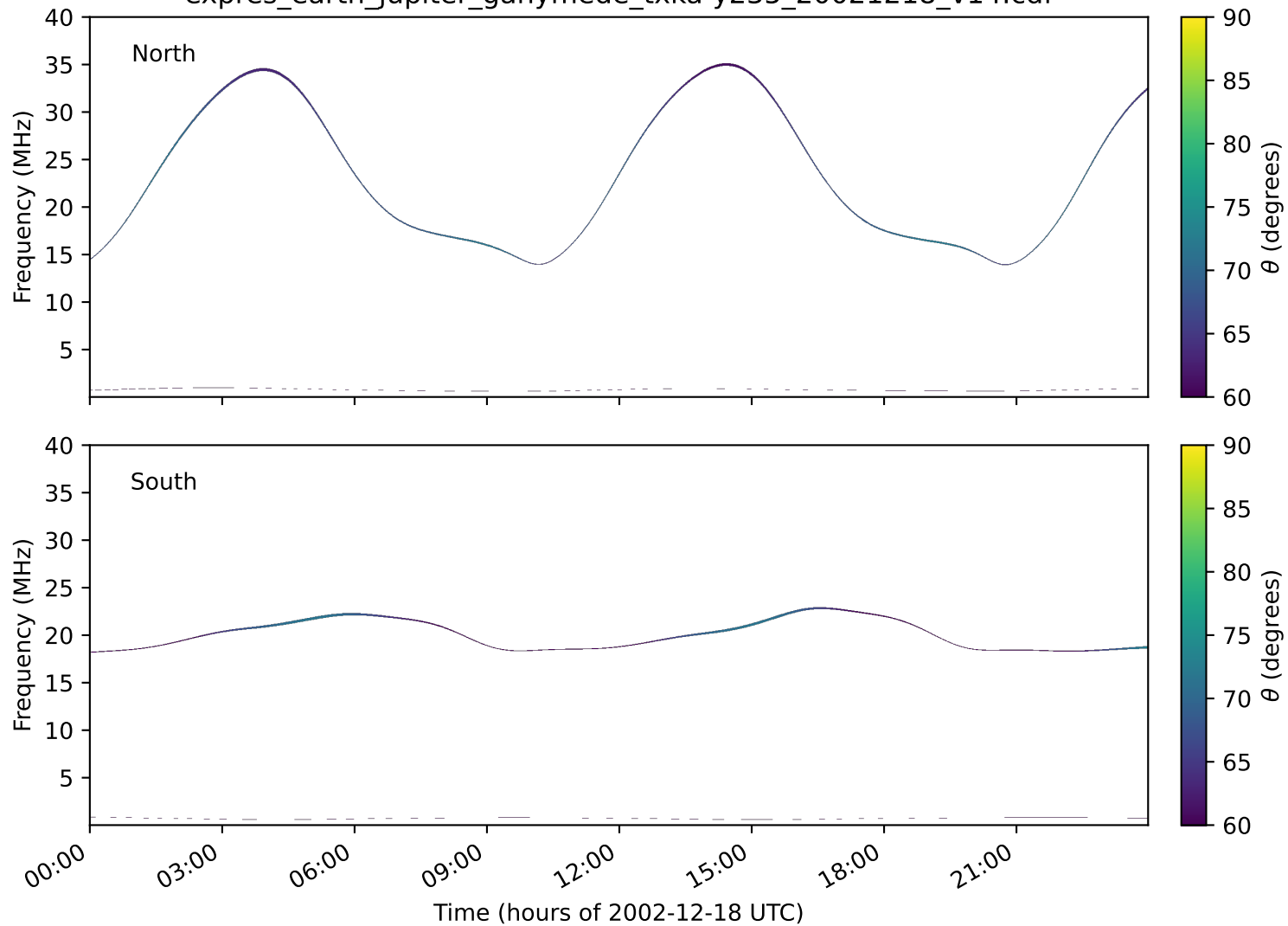
expres_earth_jupiter_ganymede_txka-y235_20021218_v14.cdf
