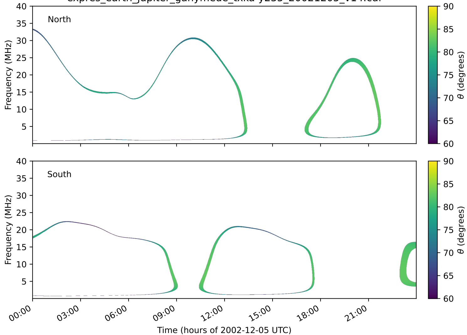
expres_earth_jupiter_ganymede_txka-y235_20021205_v14.cdf
