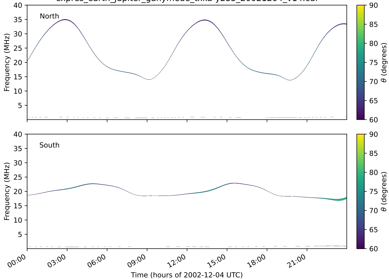
expres_earth_jupiter_ganymede_txka-y235_20021204_v14.cdf
