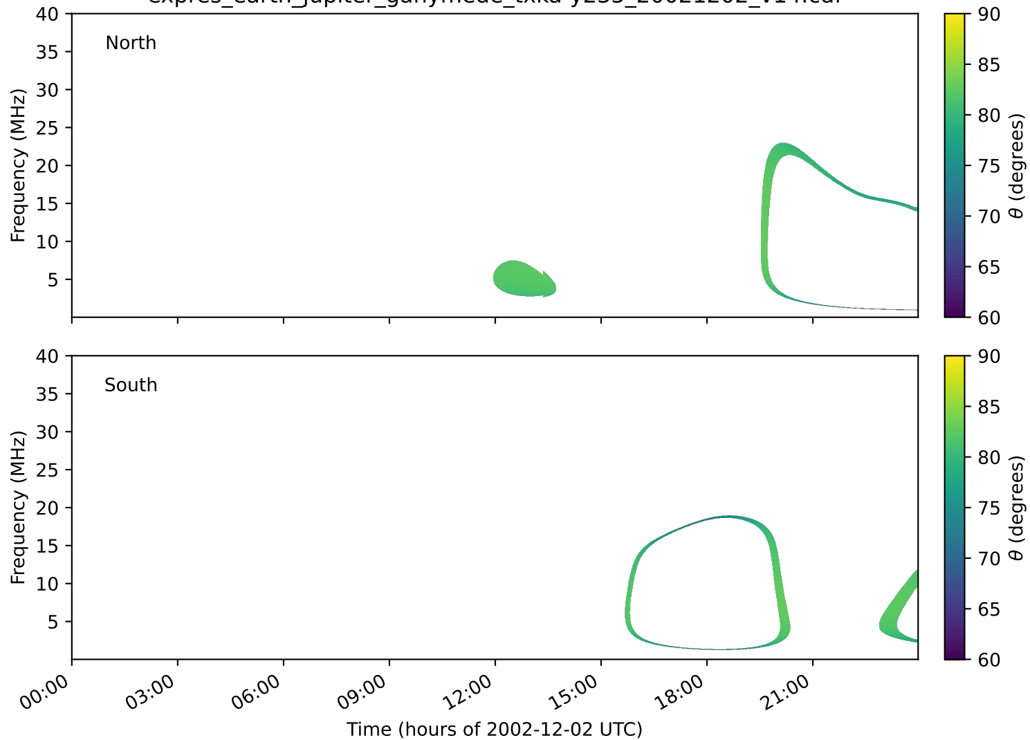
expres_earth_jupiter_ganymede_txka-y235_20021202_v14.cdf
