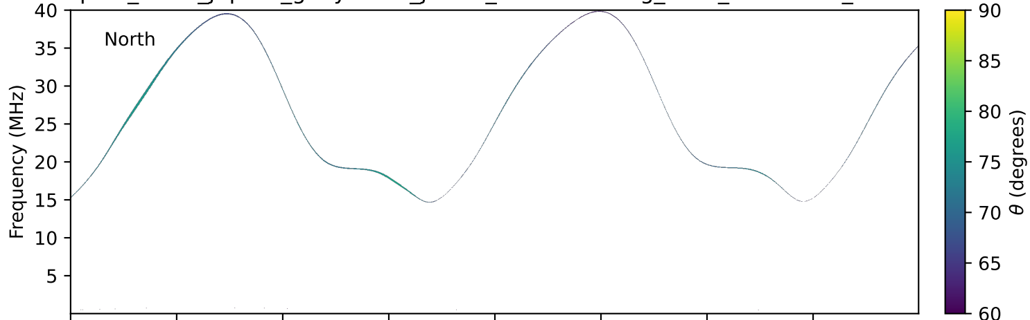
expres_earth_jupiter_ganymede_jrm33_lossc-wid1deg_3kev_20021225_v11.cdf
