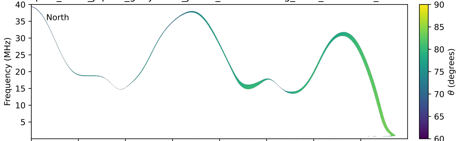
expres_earth_jupiter_ganymede_jrm33_lossc-wid1deg_3kev_20021205_v11.cdf
