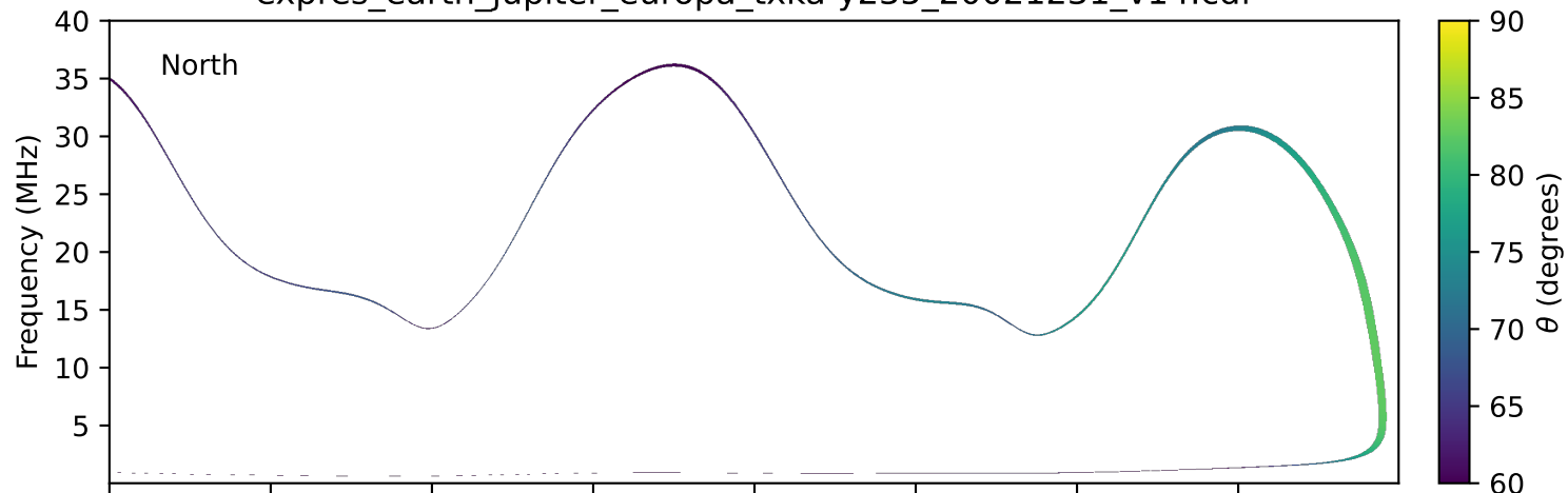
expres_earth_jupiter_europa_txka-y235_20021231_v14.cdf
