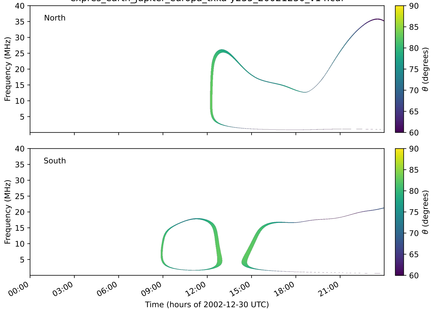
expres_earth_jupiter_europa_txka-y235_20021230_v14.cdf
