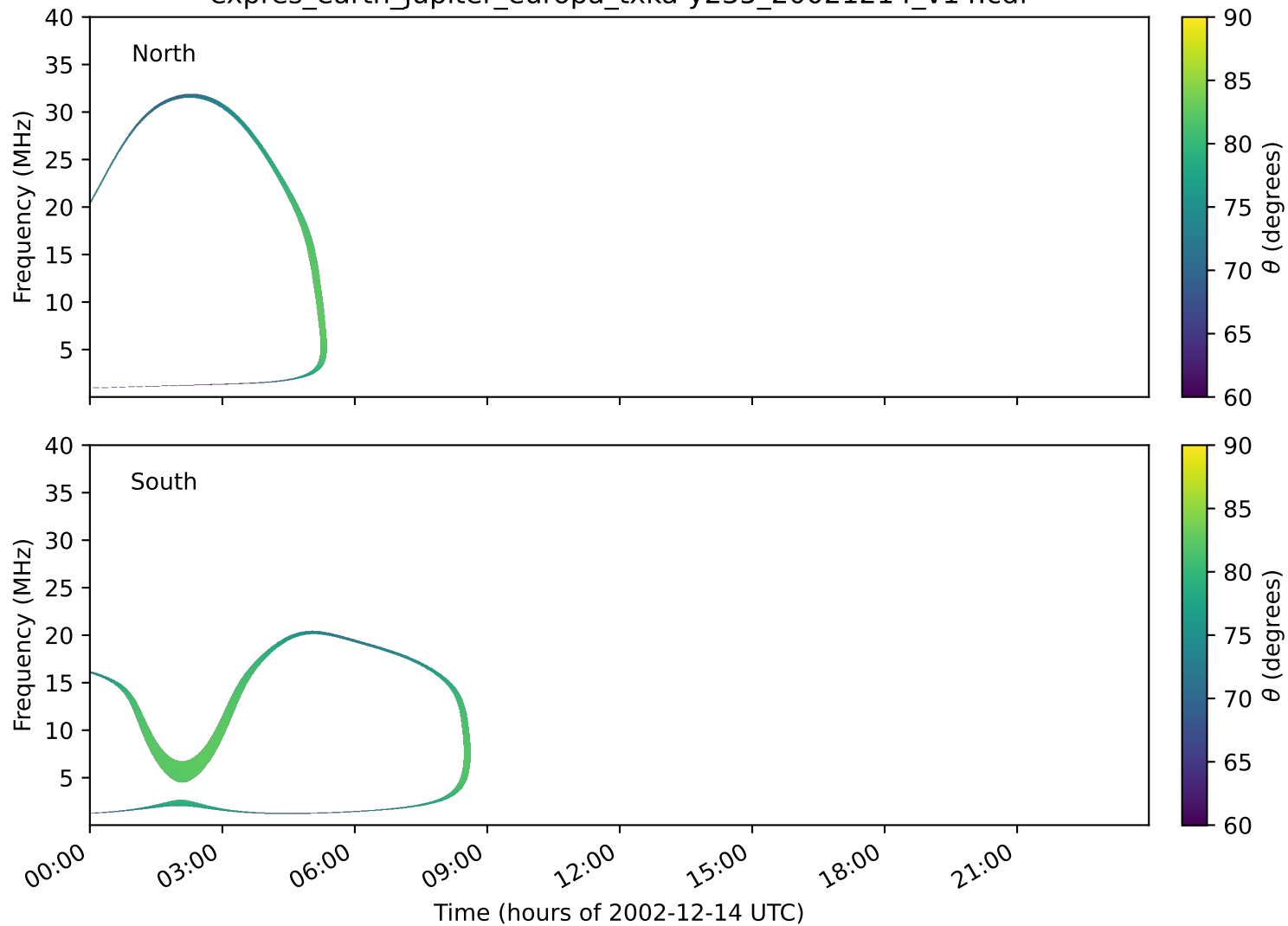
expres_earth_jupiter_europa_txka-y235_20021214_v14.cdf
