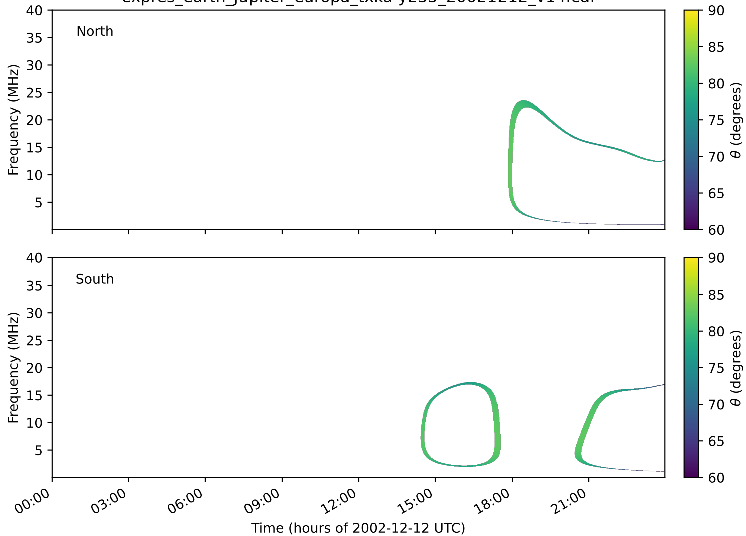
expres_earth_jupiter_europa_txka-y235_20021212_v14.cdf
