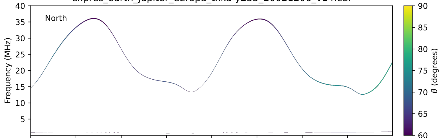
expres_earth_jupiter_europa_txka-y235_20021206_v14.cdf
