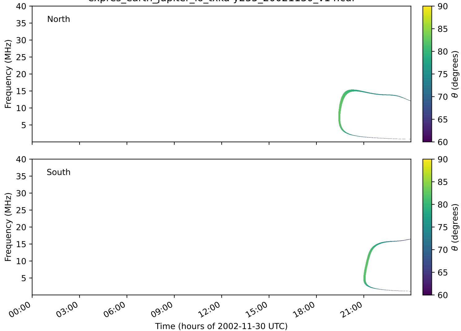
expres_earth_jupiter_io_txka-y235_20021130_v14.cdf
