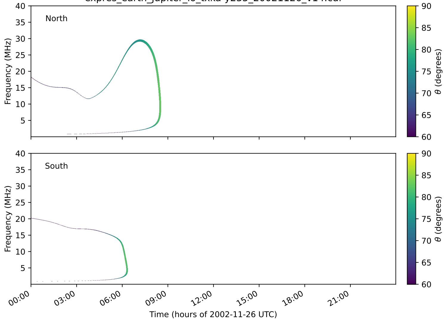
expres_earth_jupiter_io_txka-y235_20021126_v14.cdf
