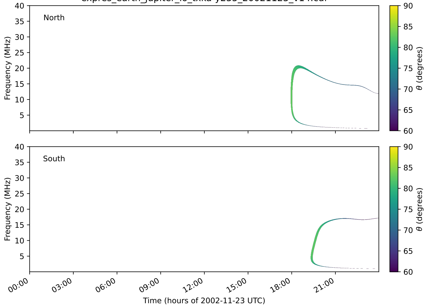
expres_earth_jupiter_io_txka-y235_20021123_v14.cdf
