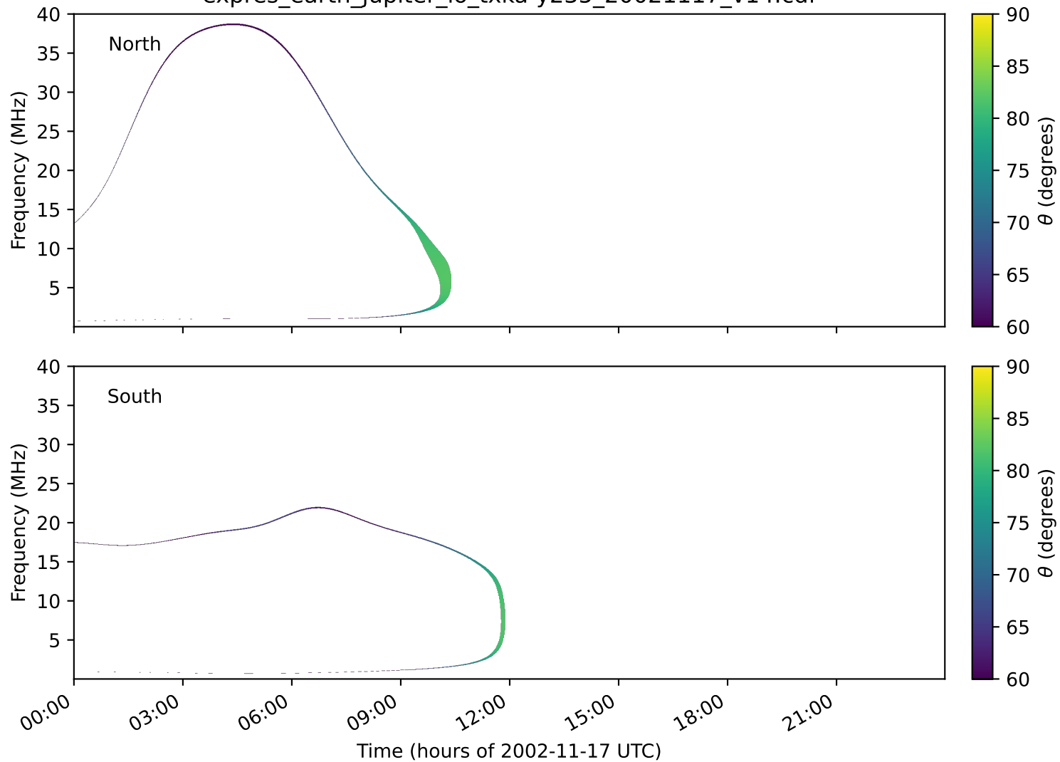
expres_earth_jupiter_io_txka-y235_20021117_v14.cdf
