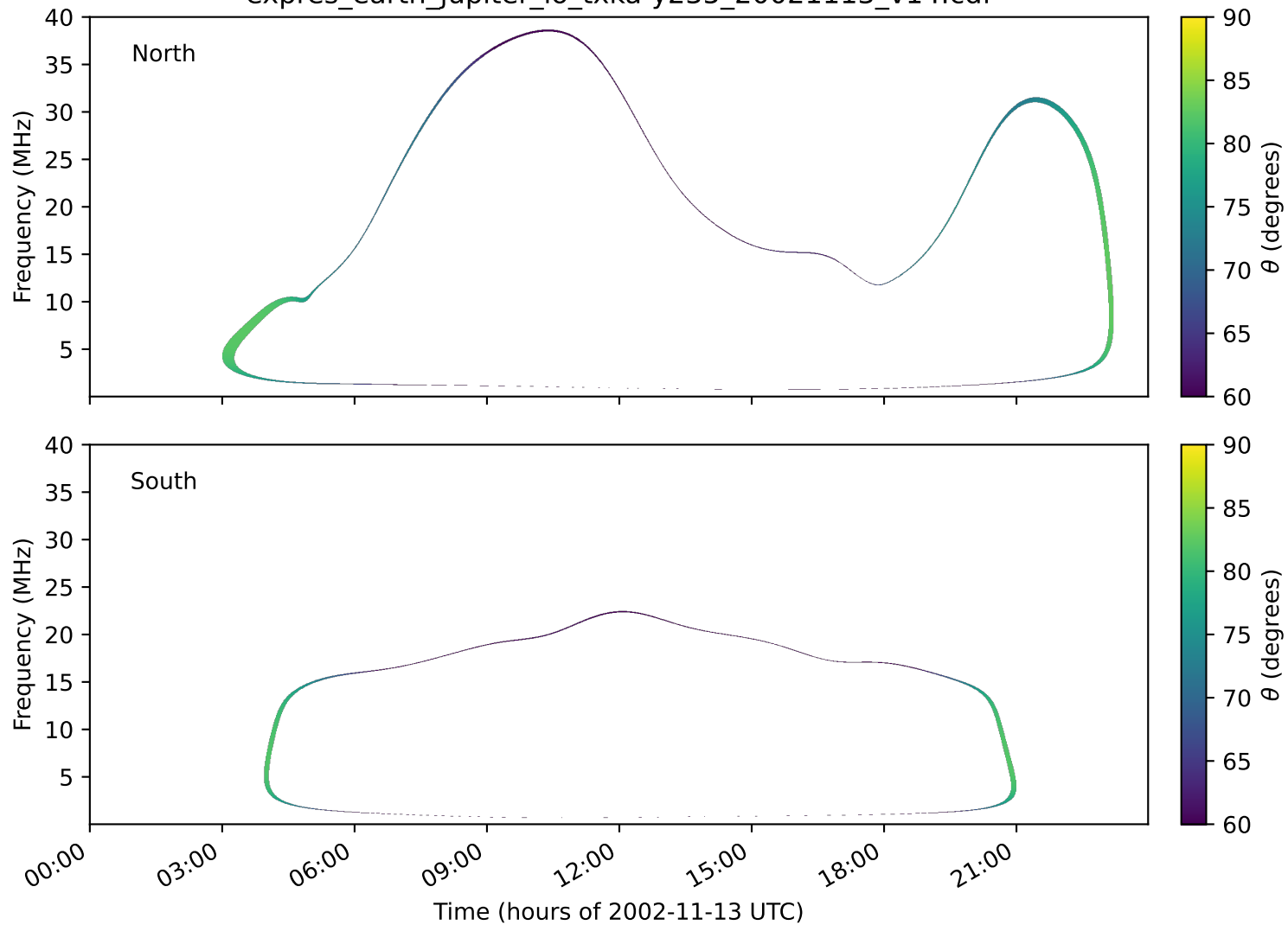
expres_earth_jupiter_io_txka-y235_20021113_v14.cdf
