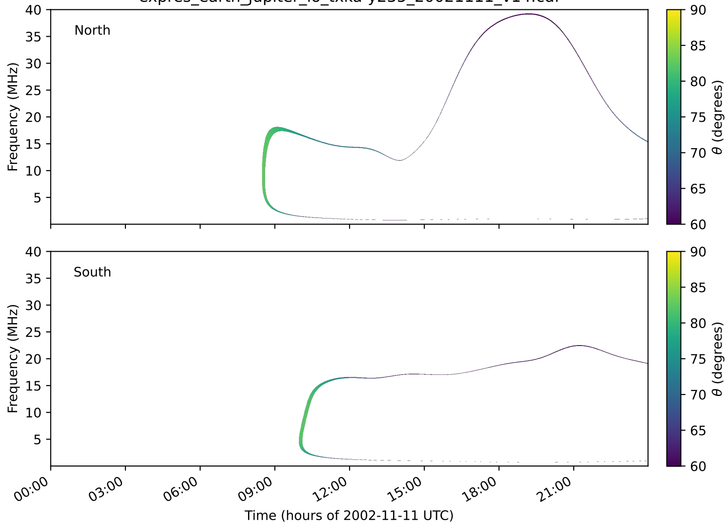
expres_earth_jupiter_io_txka-y235_20021111_v14.cdf
