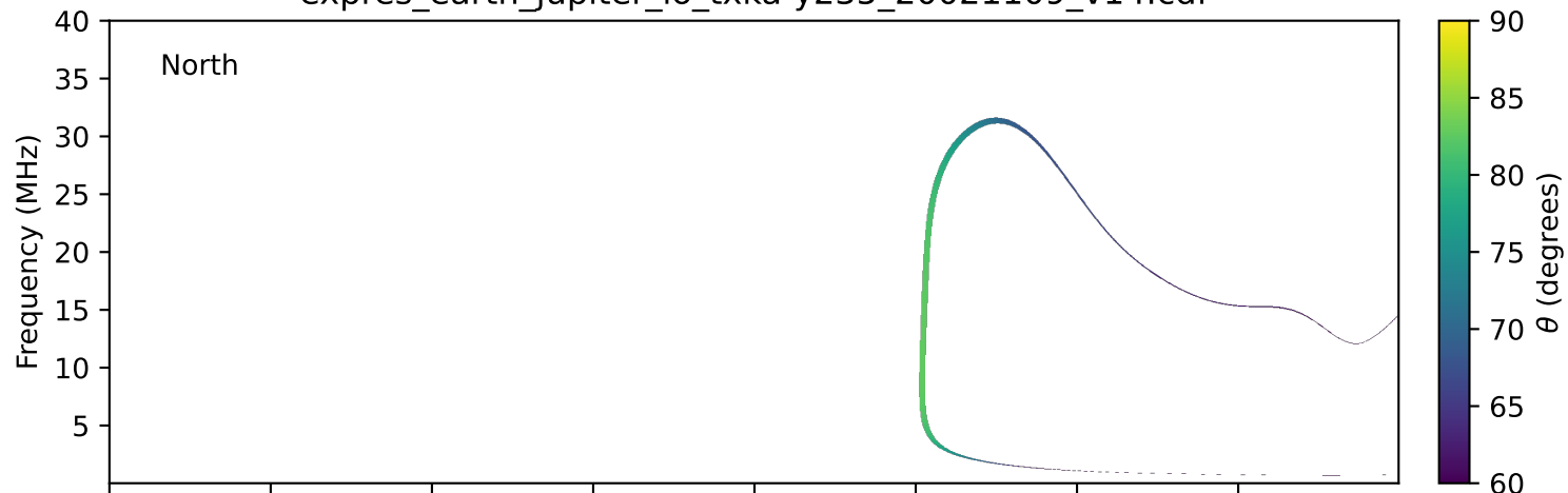
expres_earth_jupiter_io_txka-y235_20021109_v14.cdf
