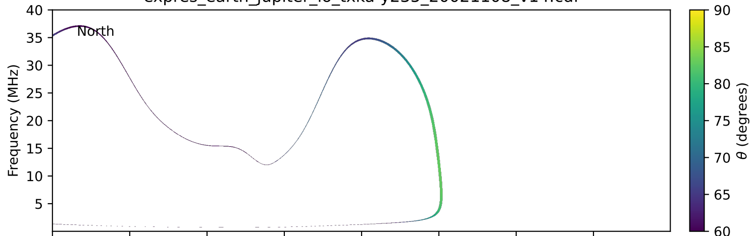
expres_earth_jupiter_io_txka-y235_20021108_v14.cdf
