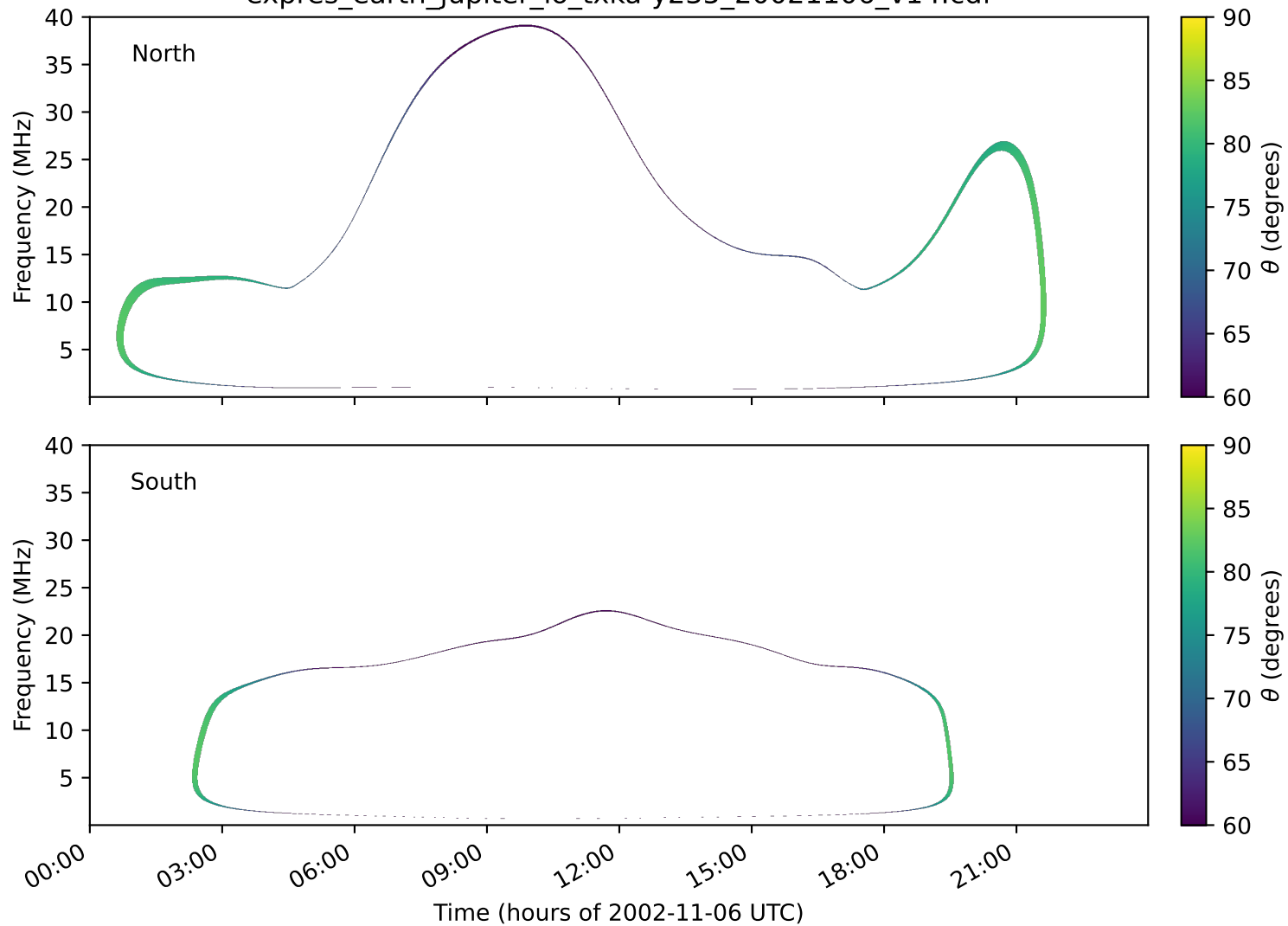
expres_earth_jupiter_io_txka-y235_20021106_v14.cdf
