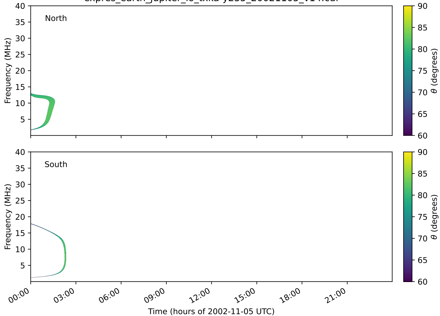
expres_earth_jupiter_io_txka-y235_20021105_v14.cdf
