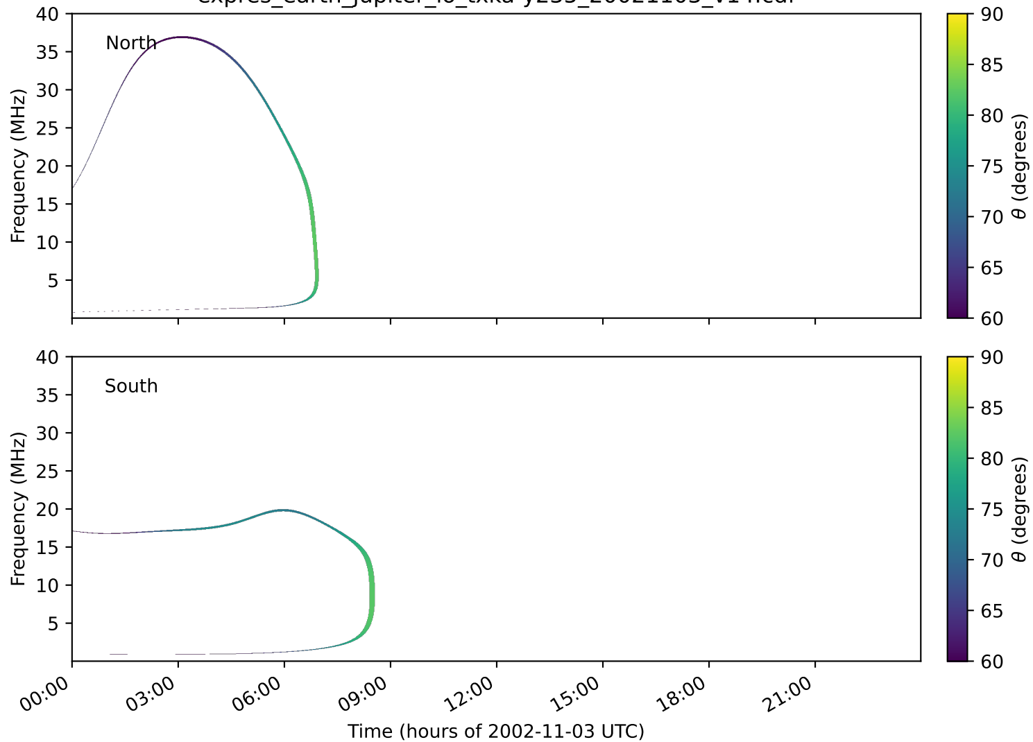
expres_earth_jupiter_io_txka-y235_20021103_v14.cdf
