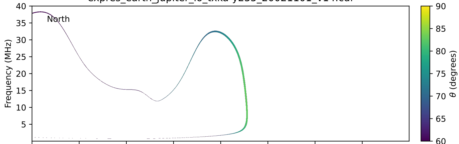
expres_earth_jupiter_io_txka-y235_20021101_v14.cdf
