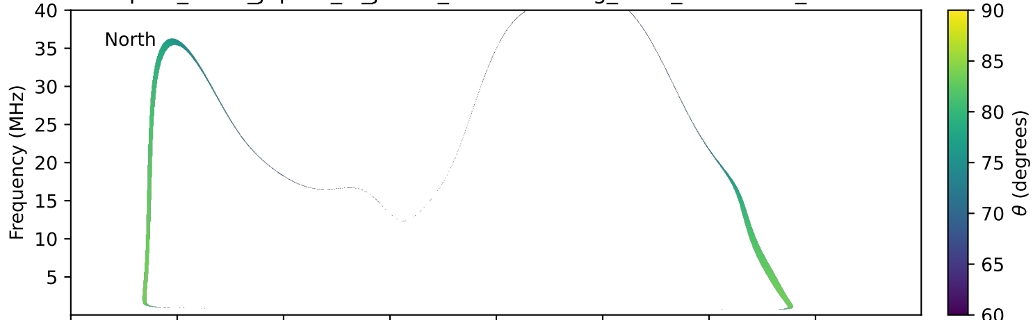
expres_earth_jupiter_io_jrm33_lossc-wid1deg_3kev_20021129_v11.cdf
