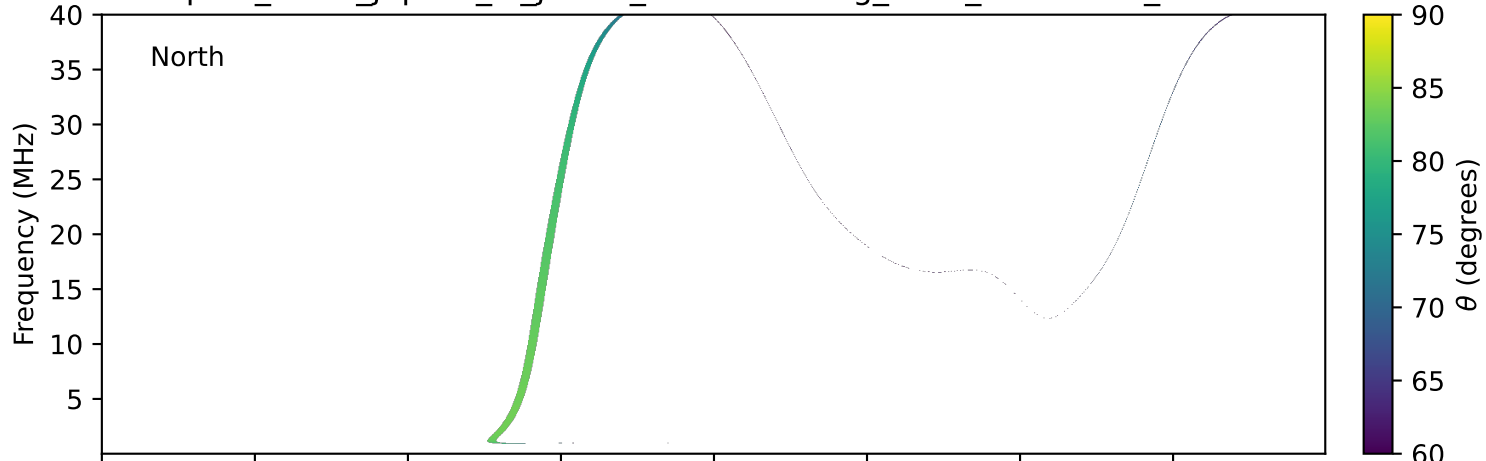
expres_earth_jupiter_io_jrm33_lossc-wid1deg_3kev_20021127_v11.cdf
