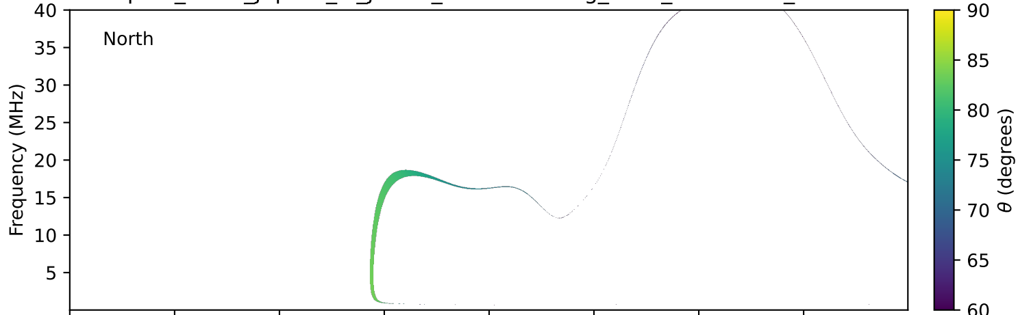
expres_earth_jupiter_io_jrm33_lossc-wid1deg_3kev_20021111_v11.cdf
