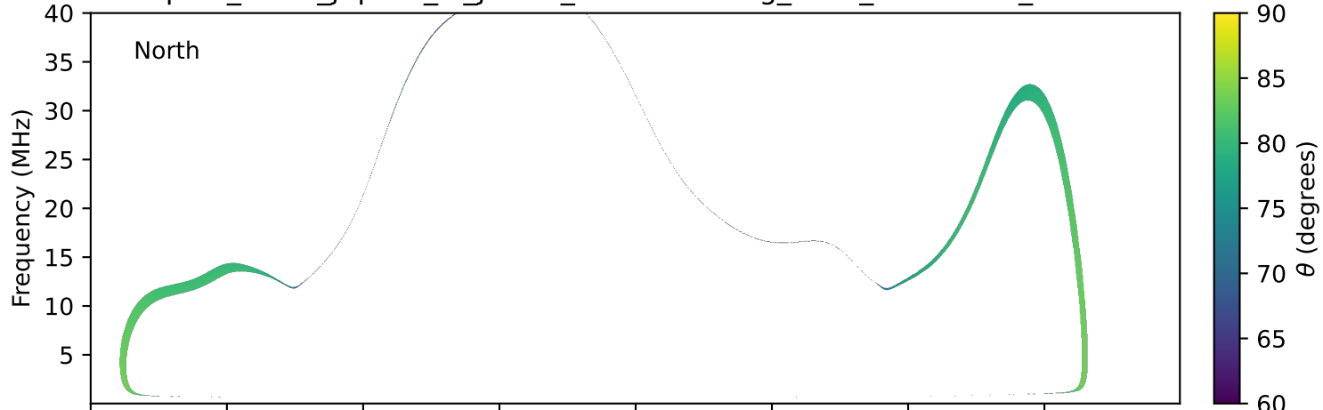
expres_earth_jupiter_io_jrm33_lossc-wid1deg_3kev_20021106_v11.cdf
