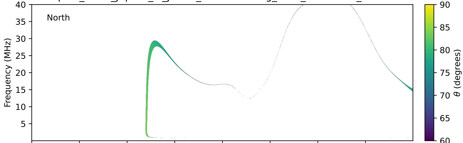
expres_earth_jupiter_io_jrm33_lossc-wid1deg_3kev_20021104_v11.cdf
