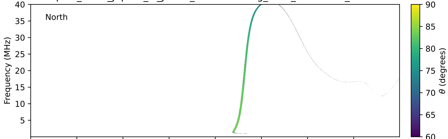
expres_earth_jupiter_io_jrm33_lossc-wid1deg_3kev_20021102_v11.cdf
