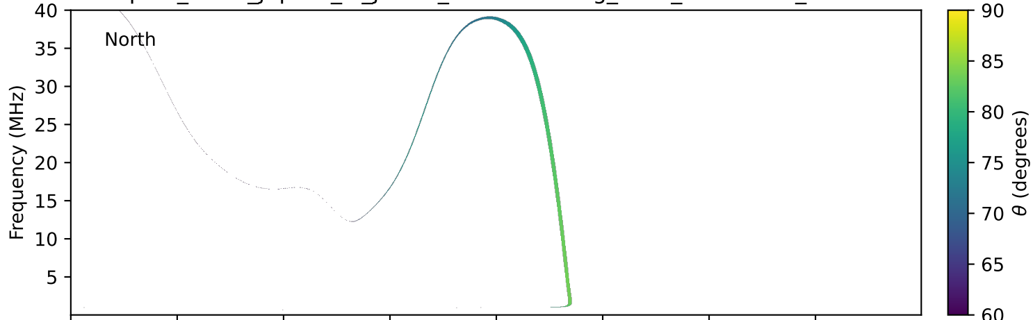
expres_earth_jupiter_io_jrm33_lossc-wid1deg_3kev_20021101_v11.cdf
