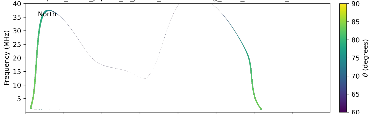
expres_earth_jupiter_io_jrm09_lossc-wid1deg_3kev_20021122_v11.cdf
