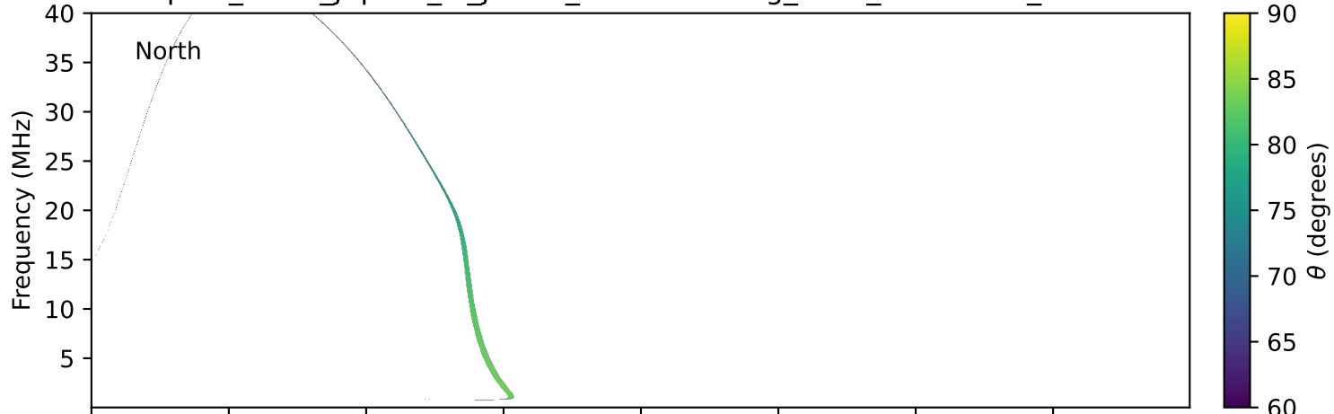
expres_earth_jupiter_io_jrm09_lossc-wid1deg_3kev_20021110_v11.cdf
