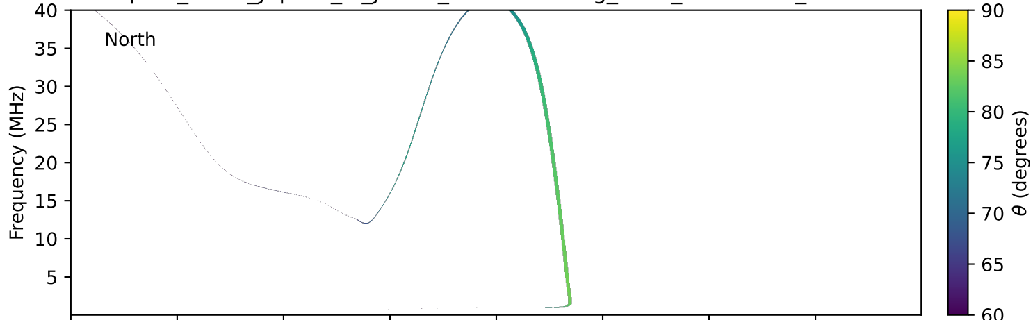
expres_earth_jupiter_io_jrm09_lossc-wid1deg_3kev_20021101_v11.cdf
