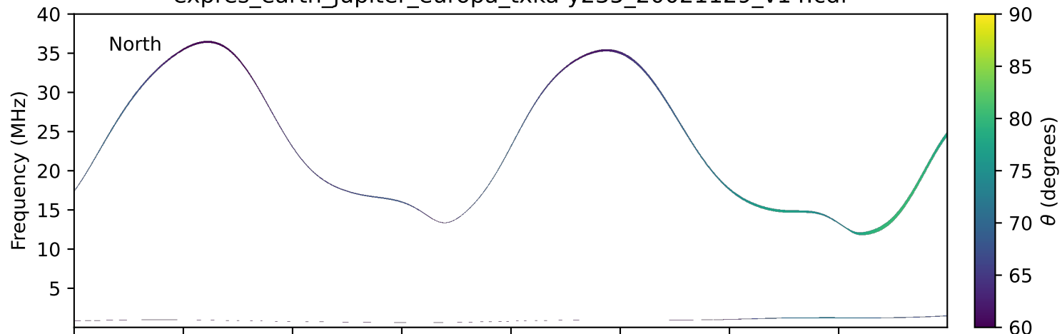
expres_earth_jupiter_europa_txka-y235_20021129_v14.cdf
