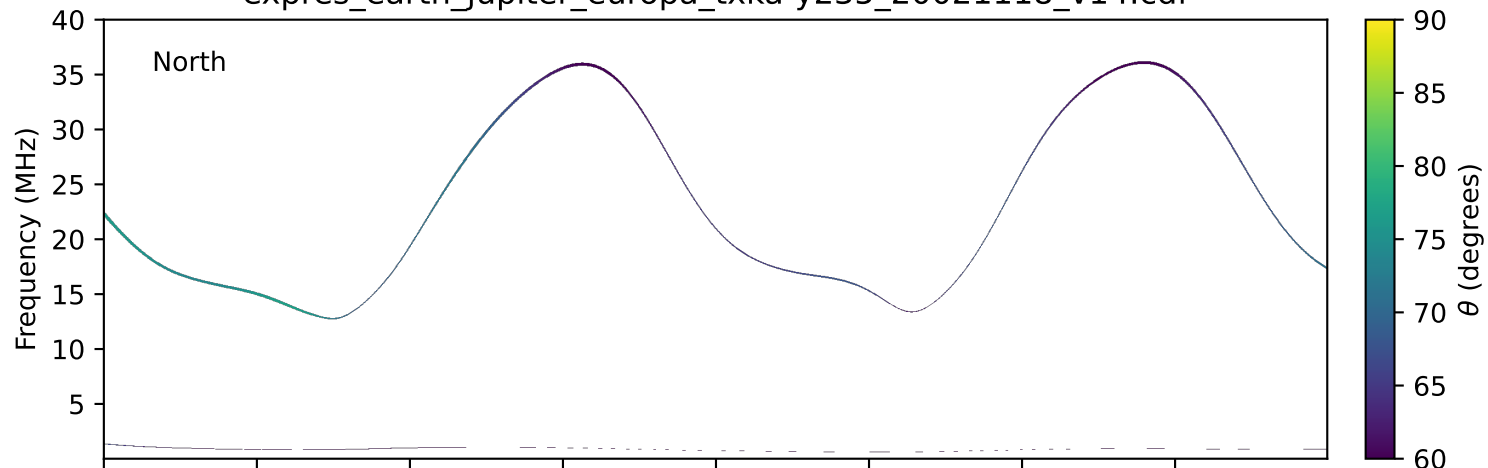
expres_earth_jupiter_europa_txka-y235_20021118_v14.cdf
