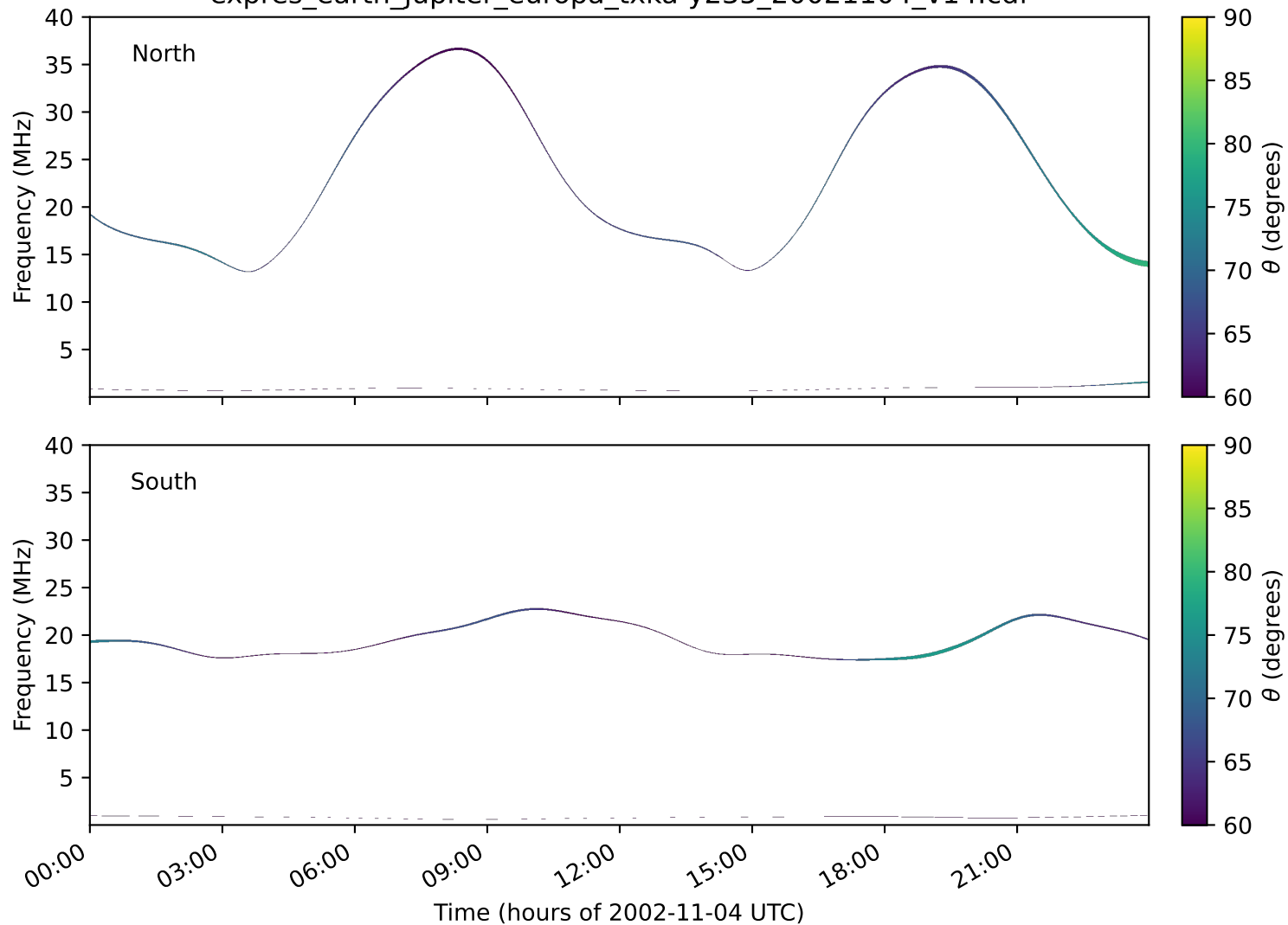
expres_earth_jupiter_europa_txka-y235_20021104_v14.cdf
