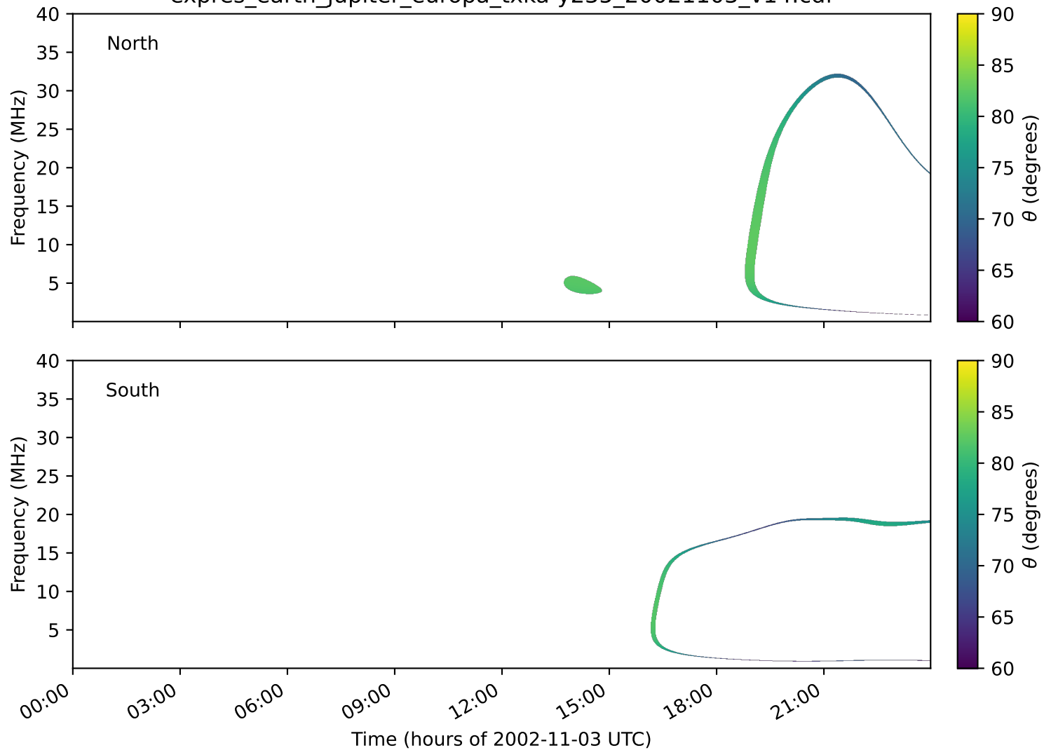
expres_earth_jupiter_europa_txka-y235_20021103_v14.cdf
