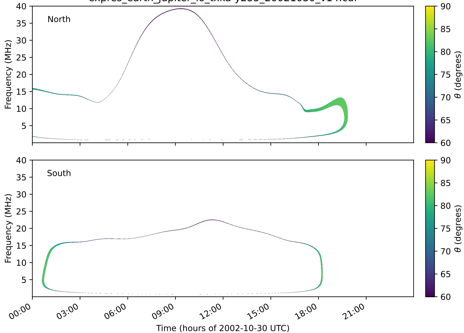
expres_earth_jupiter_io_txka-y235_20021030_v14.cdf
