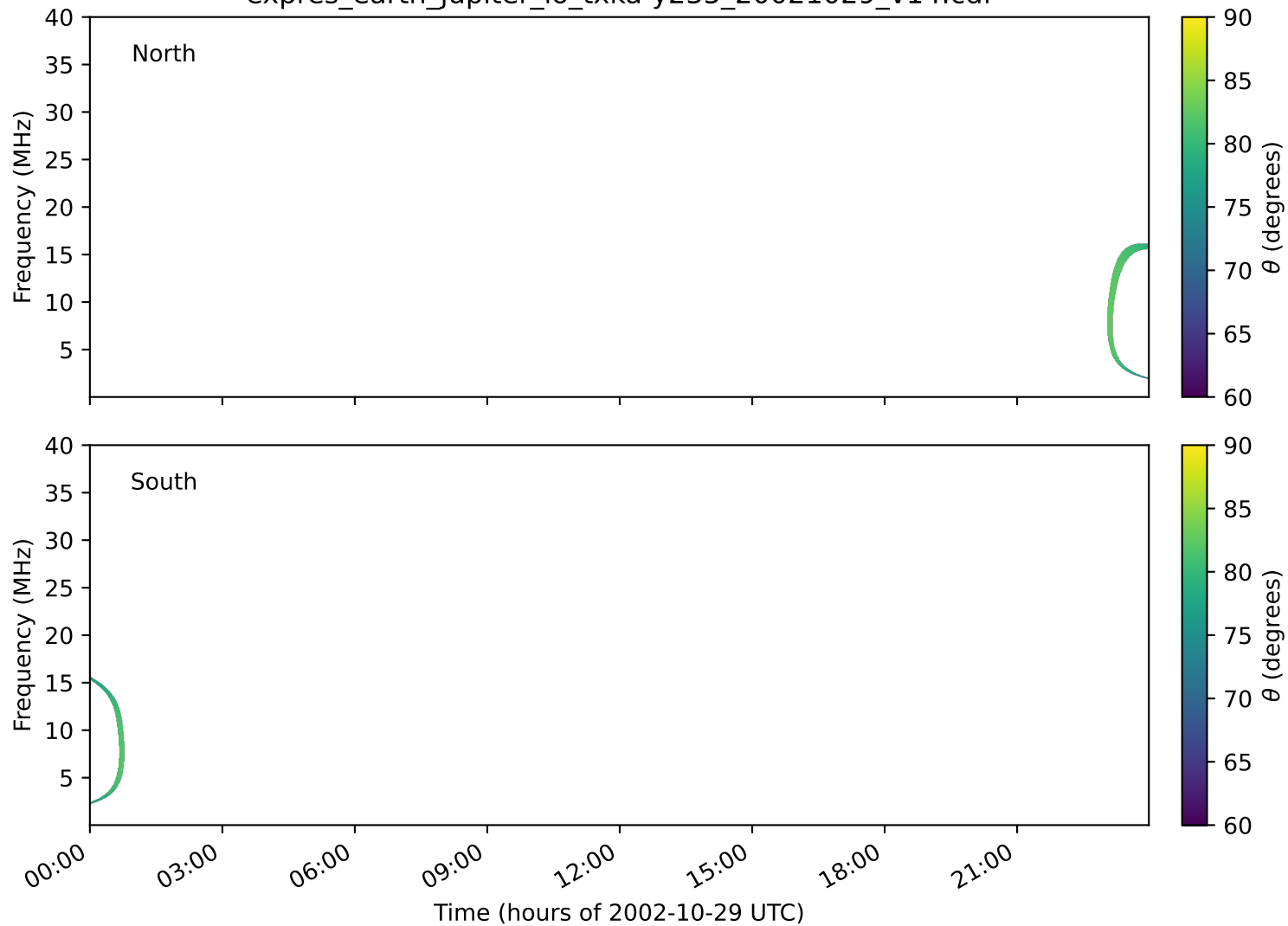
expres_earth_jupiter_io_txka-y235_20021029_v14.cdf
