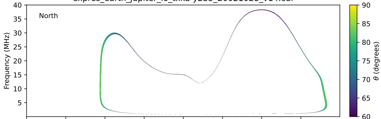
expres_earth_jupiter_io_txka-y235_20021028_v14.cdf
