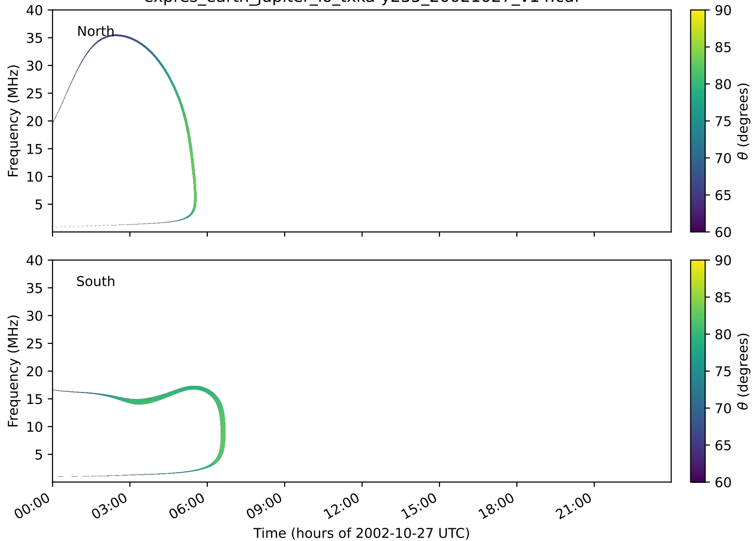
expres_earth_jupiter_io_txka-y235_20021027_v14.cdf
