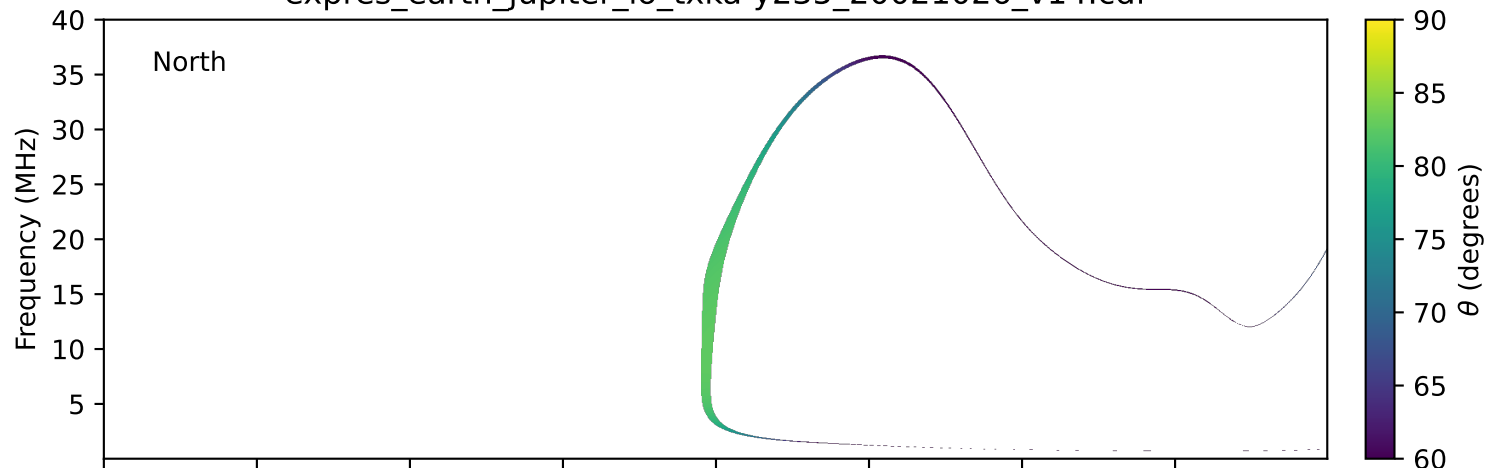
expres_earth_jupiter_io_txka-y235_20021026_v14.cdf
