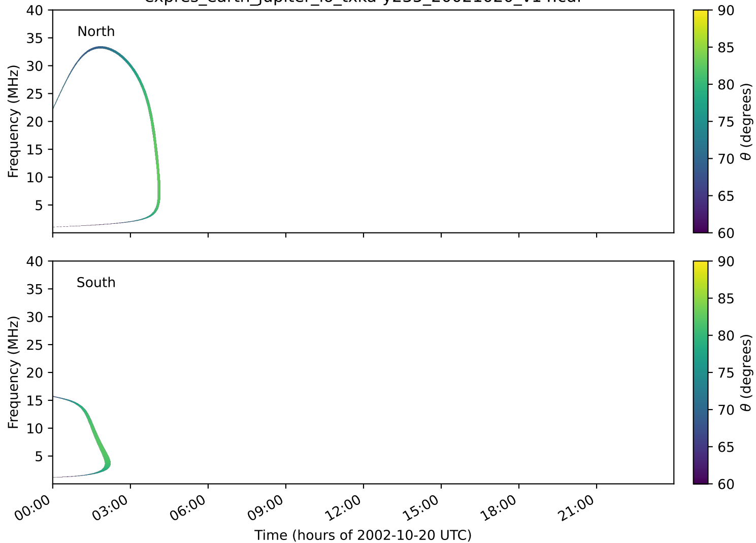
expres_earth_jupiter_io_txka-y235_20021020_v14.cdf
